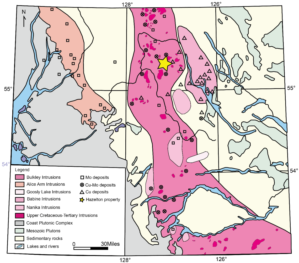
Figure 1: Age and Distribution of Upper Cretaceous to Tertiary Intrusions and Porphyry Deposits in West Central B.C. (Modified after Carter, 1974)
